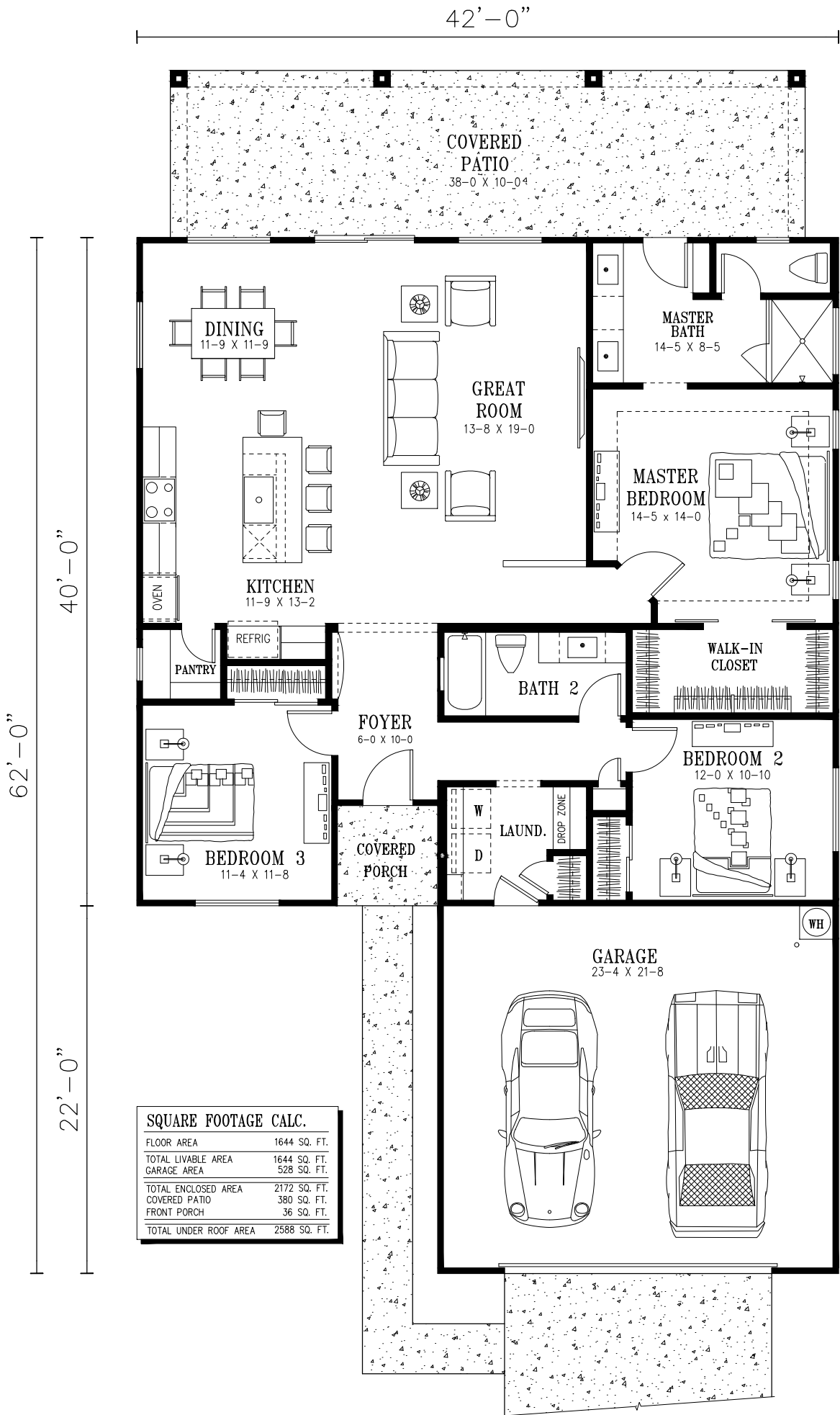
1600 FLOOR PLAN with Rear Bath and Deluxe Kitchen
