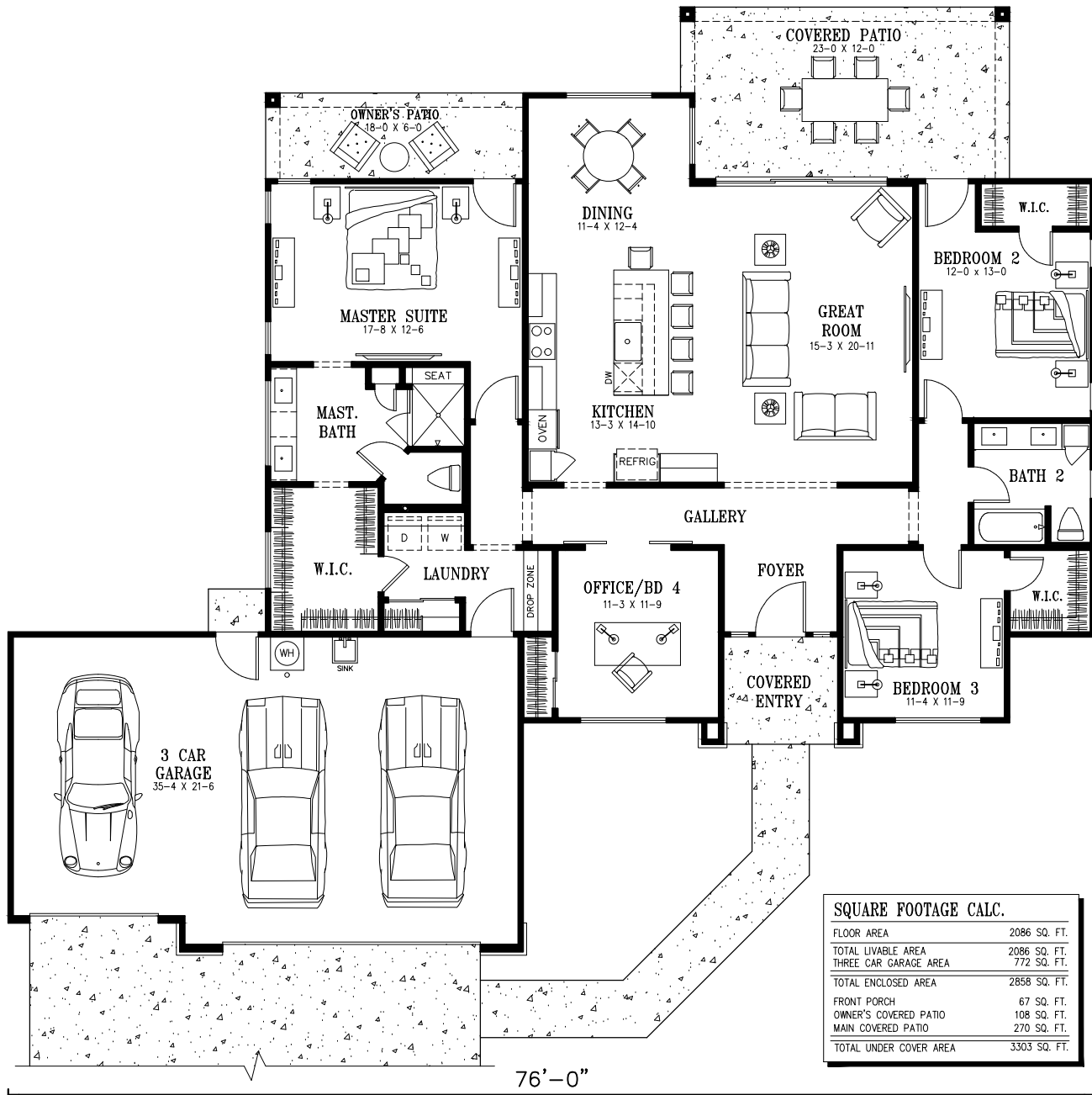
2020 FLOOR PLAN w/3 CAR GARAGE
